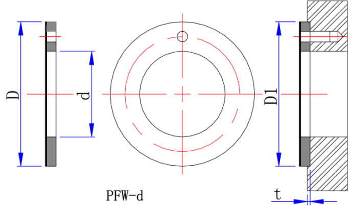
PFW THRUST WASHERS STANDARD
